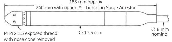
Installation drawing
